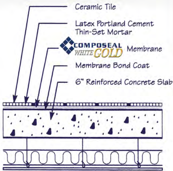
Figure 2 COMPOSEAL WHITE GOLD in thin-set tile installation over 6" reinforced concrete slab above suspended ceiling.
